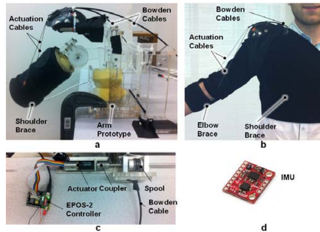
Figure 3. a) Soft-Orthotic System Prototype. b) User wearing the soft-orthotic device. c) Actuation and controller located on table and transmitted by bowden cables to minimize weight. d) IMU sensor to measure user's posture
