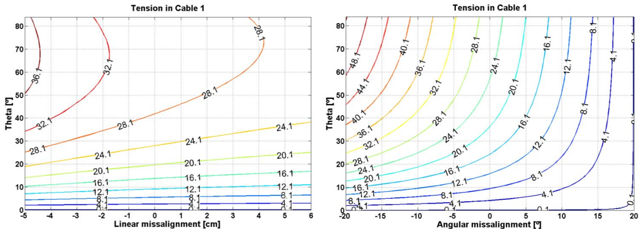
Figure 5. Two cables are needed to compensate for angular and linear misalignments (Brace misalignment parameters: r, \alpha ). a) Tension required in cable 1 to compensate for linear missalignments. Here T_2 = T_1 . b) Tension required in cable 1 to compensate for angular misalignments. Here T_1(\alpha) = T_2(-\alpha) .
