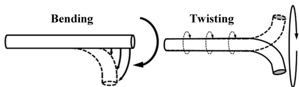
Fig. 18. Additional actuated DOF. (Left) Bending of the catheter tip generated by pull wires inside of the guidewire. (Right) Twisting of the catheter achieved by rotating the guidewire at the drive system module.
